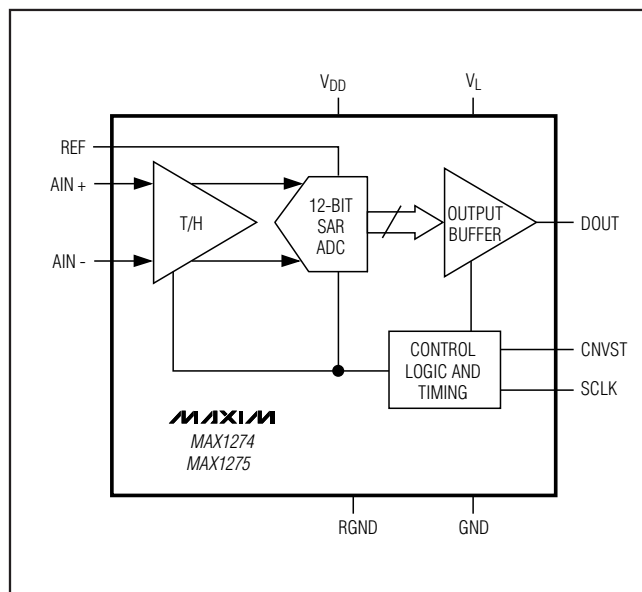
Figure 3. Functional Diagram
